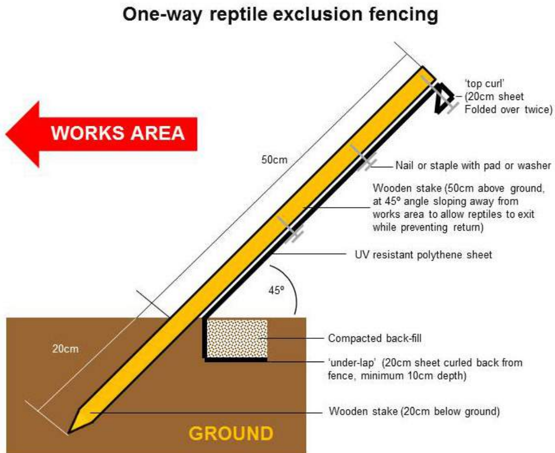
Figure 4. Example specification for one-way reptile fencing.
